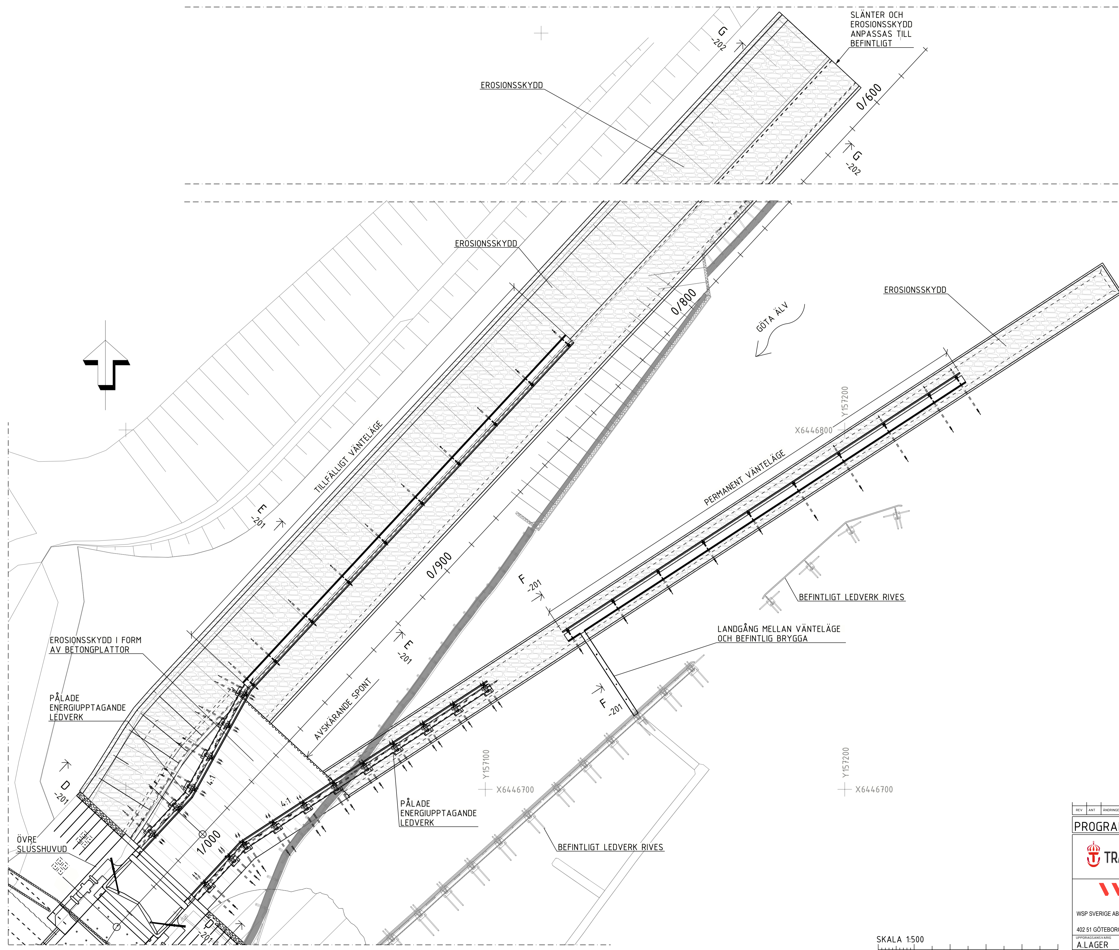
PLAN 1:500
