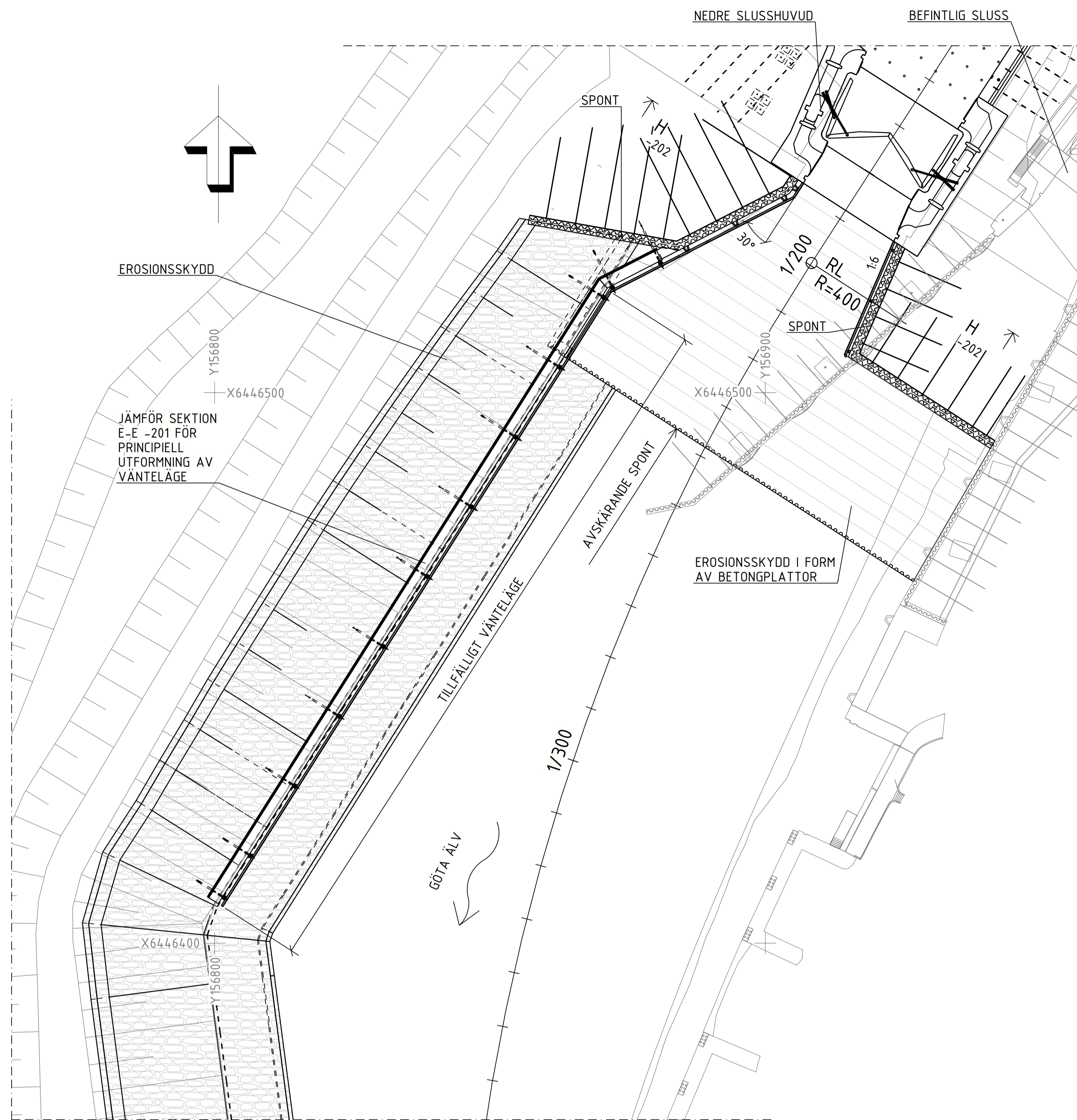
PLAN 1:500
